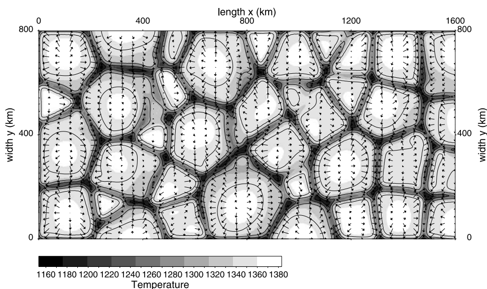
Figure 3. Initial temperature and horizontal velocity field on an horizontal plane at 104 km depth (mean value of the lithospheric depth). Maximum velocity is 2.7 \text{ cm yr}^{-1} .
