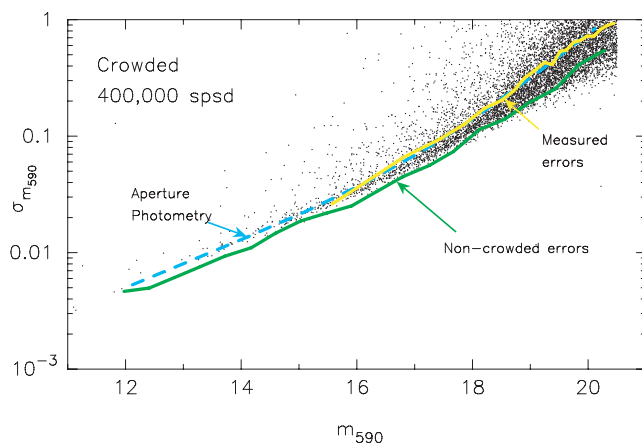
Figure 11. Various single transit error estimates: the dashed (blue) line is for the case of aperture photometry (equation 2); the solid (green) line for the case of PSF fitting photometry using accurate positional information from astrometric processing in a non-crowded field; and the shorter (yellow) line on the right above the green line shows the same for a crowded-field (400 000 stars \text{deg}^{-2} ). The black dots are the formal errors from the PSF fitting solution in the crowded case. ( m_{590} is the magnitude for a representative MBP passband at 590 nm.)
