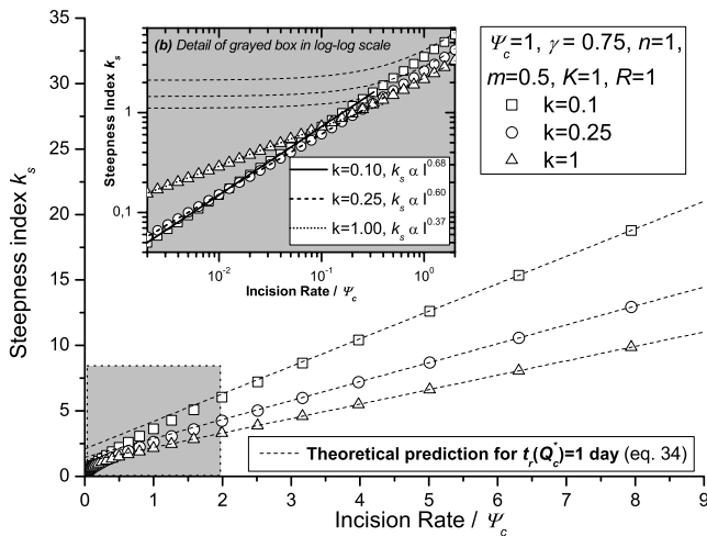
Figure 9. Numerical solutions for the relationship between channel steepness and steady state incision rate for three discharge variability coefficient k . Insert is a log-log plot of the same data focusing on small incision rates and highlighting the power law relationship predicted by equation (35). Units are arbitrary. For low incision rates the steepness-uplift power law exponent \phi increases with the runoff variability (see equation (37)). For large incision rate (compared to the threshold parameter \psi_c ) the relationship corresponds to the predictions of a constant effective discharge model ( t_r(Q_c^*) = 1 day). In this regime (and for \gamma \leq 1 ) the steady state steepness increases with runoff variability for a given incision rate. This is the opposite for low incision rates. See color version of this figure in the HTML.
