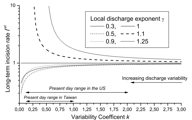
Figure 2. Variation of long-term incision rate with variability coefficient k for different values of \gamma .
