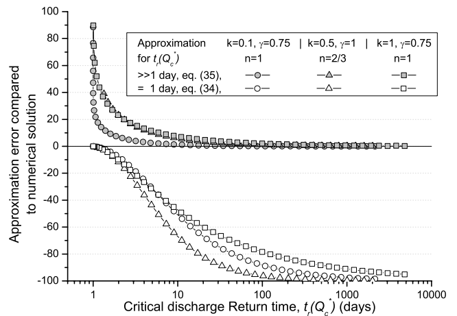
Figure 8. Comparison of the quality of the asymptotic approximation of the steepness index using equations (34) (constant discharge model) and (35) (asymptotic discharge model for large Q_c^* ) as a function of the return time of Q_c^* for various incision and discharge condition parameters.
