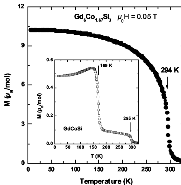
Fig. 1. Temperature dependence of the magnetization, measured with an applied field \mu_0 H = 0.05 T, of \text{Gd}_6\text{Co}_{1.67}\text{Si}_3 and GdCoSi (inset).
