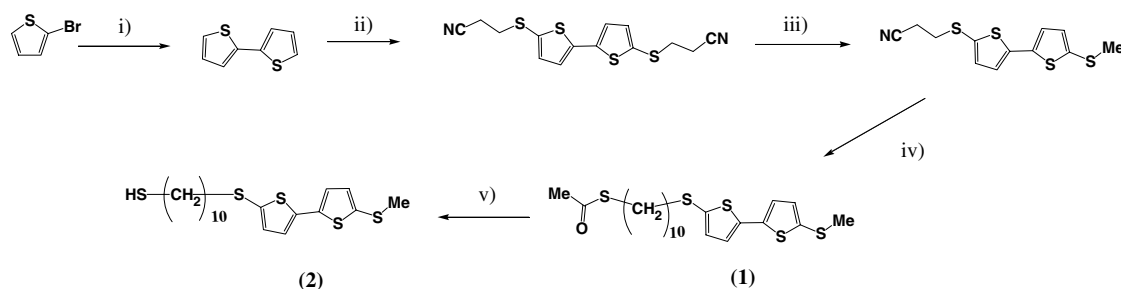
Scheme 1. Synthesis of alkane-thiol ( 2 ). Reagents and conditions: (i) Magnesium, NidpppCl 2 , Et 2 O, reflux; (ii) nBuLi, sulphur and 2-bromopropionitrile, THF, room temperature; (iii) Cesium hydroxide (1 equiv.) and methyl iodide, DMF/MeOH, room temperature, 2 h; 18 (iv) Cesium hydroxide (2 equiv.) and 10-thioacetate-bromodecane, DMF/MeOH, room temperature, overnight; (v) Cesium hydroxide, THF, room temperature, 3 h.
