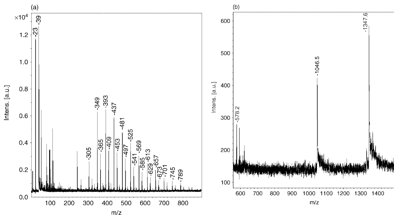
Figure 2. (a) Positive ion DIAMS mass spectrum of two poly(ethyleneglycol) mixtures with nominal molecular weights centered around 400 and 600. The peaks of Na + ( m/z 23) and K + ( m/z 39) are depicted in the mass spectrum with the alkali metal adducts of PEG, i.e. [M + Na] + and [M + K] + . (b) Expansion of the positive ion DIAMS mass spectrum of a peptide mixture. Signals at m/z 578.2, m/z 1046.5 and m/z 1347.6 correspond to the [M + Na] + of the leucine enkephaline ( 2 \times 10^{-10} mol deposited on the plate), the [M + H] + of the angiotensin II ( 8 \times 10^{-11} mol deposited on the plate) and the [M + H] + of the substance P ( 8 \times 10^{-11} mol deposited on the plate), respectively.
