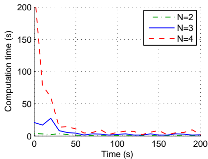
Fig. 5. Computation time versus simulation time ( N = 2, 3, 4 ) with partial enumeration
