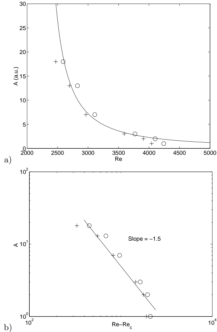
Figure 16. a) Stability curve f(Re) where the amplitude is considered to be proportional to the number of spots, b) the same in log-log scale where the best fit gives Re_c = 2140 and \alpha = -1.5 . f(Re) is determined for h = 2.0 mm and \Omega = 150 rpm (+) and for h = 2.6 mm and \Omega = 110 rpm (o).
