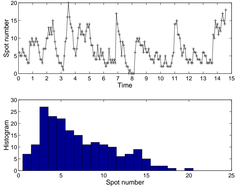
Figure 7. top: Temporal series (time unit is the disc rotation period) of spot number for \Omega = 55 rpm and h = 3.1 mm. Strong intermittency is observable with some burstings of groups of spots. bottom: Histogram of the temporal series that shows a Poisson like distribution of the spot occurrence.
