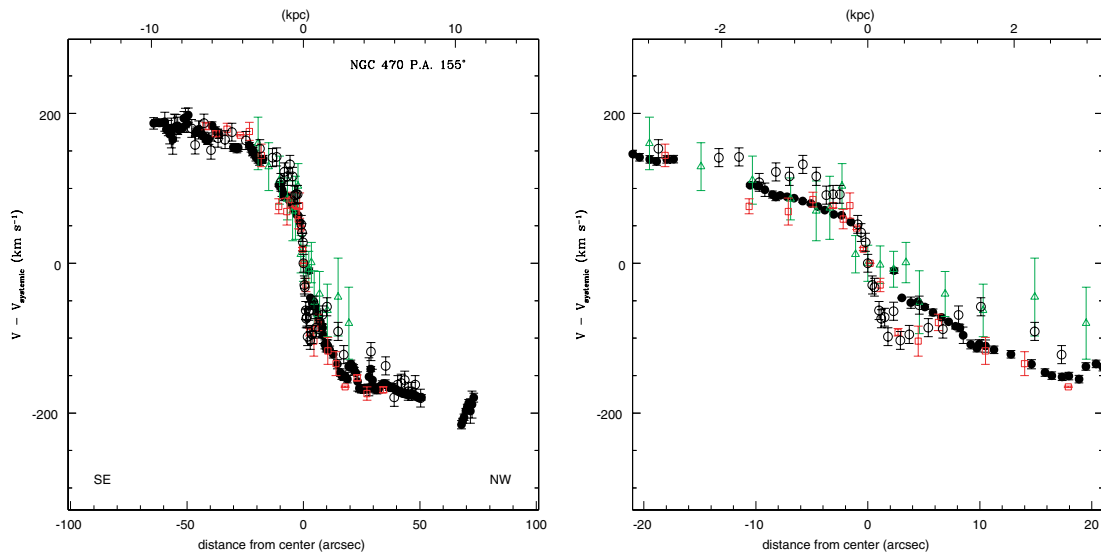
Figure 7. Left-hand panel: comparison between our H \alpha velocity profile (full circles) along PA = 155° and observations obtained by Vega Beltran et al. (2001) [the gas component (O III line: open circles), stars (open squares)] and Héraudeau et al. (1999) (stars: open triangles). Right-hand panel: enlargement of the central 20 arcsec.
