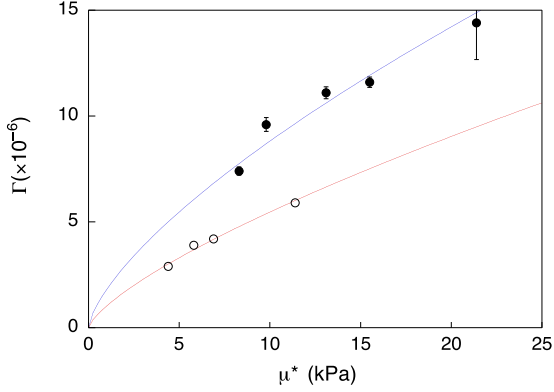
Fig. 7. \Gamma vs. \mu^* for gels from series B ( \phi = 0 , various thermal histories). c = 15 wt% (full dots); c = 10 wt% (open circles). The curves are guide for the eye.
