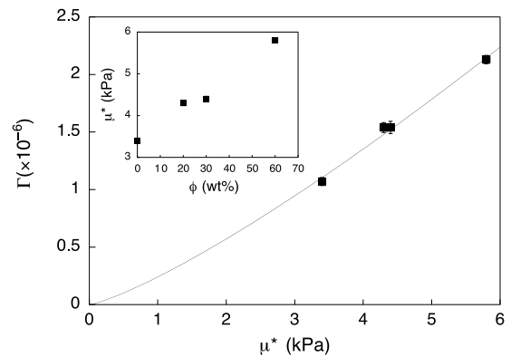
Fig. 5. Rate sensitivity \Gamma = d\mathcal{G}/d(\eta_s V) vs. \mu^* for the samples of series A. The line is the best power law fit \Gamma \sim \mu^{*1.2} . Insert shows that increasing the glycerol content stiffens the gel.
