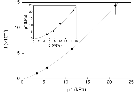
Fig. 8. \Gamma vs. \mu^* for gels from series C ( \phi = 0 , various gelatin concentrations). Insert shows \mu^* vs. c . The full lines are the power law fits (see text).
