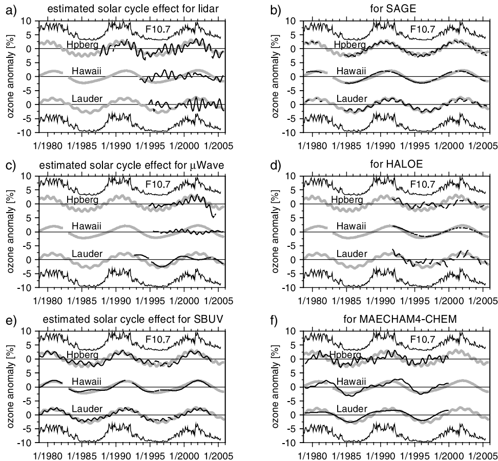
Figure 7. Estimates of ozone anomalies related to the 11-year solar cycle, for three selected stations. Note that the solar cycle estimate is for relative ozone anomalies, averaged from 35 to 45 km altitude. The different panels show results for the different data sets. Results for the all instrument average data set have been underlaid at each station (thick grey line). Thin curves at top and bottom give solar flux at 10.7 cm. Figure 7f compares results for the MAECHAM4-CHEM simulation with the average observed data set.
