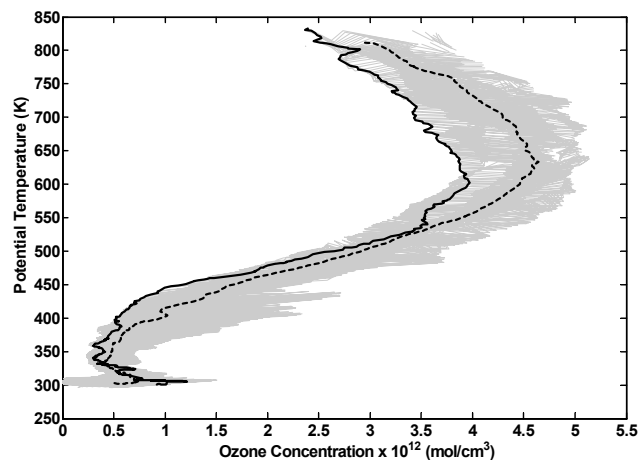
Fig. 2. Ozone concentration profile as obtained from ozonesonde measurements over Irene (25.5° S, 28.1° E) on 15 May 2002 (solid line) compared to the May profiles from 1999 to 2005 (in grey) and the corresponding mean profile (dashed line).
