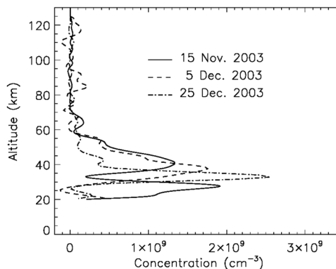
Figure 2. NO 2 measurements by GOMOS at the end of 2003, inside the Arctic Circle (latitude 72° ± 1°). No increase is detected in the mesosphere.
