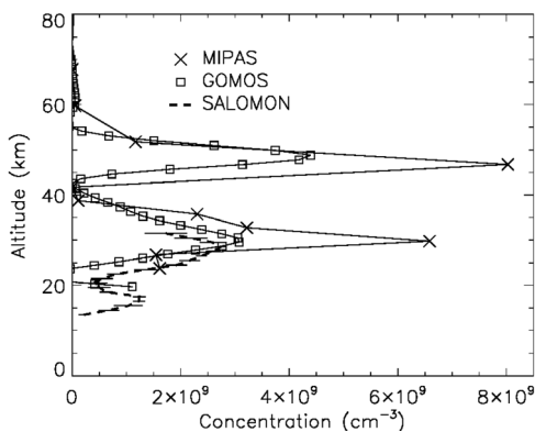
Figure 1. Typical NO 2 profile obtained in the stratosphere above Scandinavia on March 4, 2004, around 22:00 UT by GOMOS, MIPAS and balloon-borne SALOMON instrument. The unrealistic GOMOS data below 20 km are removed.
