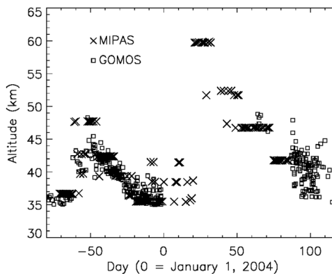
Figure 3. Evolution of the altitude of the upper NO 2 maximum concentration, from October 2003 to April 2004, using GOMOS and MIPAS data for latitude higher than 65°N. The poor vertical resolution of MIPAS induces artificial steps.
