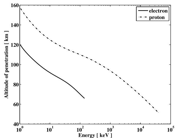
Figure 6. Altitude of penetration of precipitating particle as a function of the energy, assuming a monoenergetic beam. The curve for electrons (full lines) has been obtained using TRANSCAR ionospheric model and the curve for protons (dashed lines) is derived from NIST PSTAR database.
