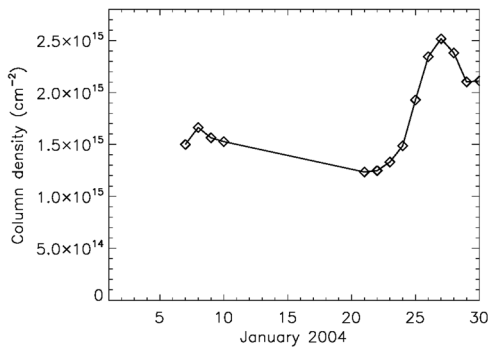
Figure 4. Vertical column density of NO 2 from ground-based UV-visible spectrometer SAOZ at Sodankyla, Finland.
