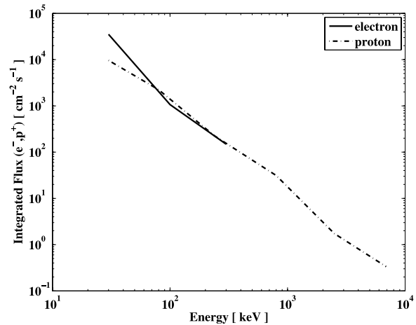
Figure 5. Integrated flux for electrons (full line) and protons (dashed line) averaged over POES-15, POES-16 and POES-17 satellites for measurements at geographic latitude higher than 78° in both hemispheres, on January 22, 2004.
