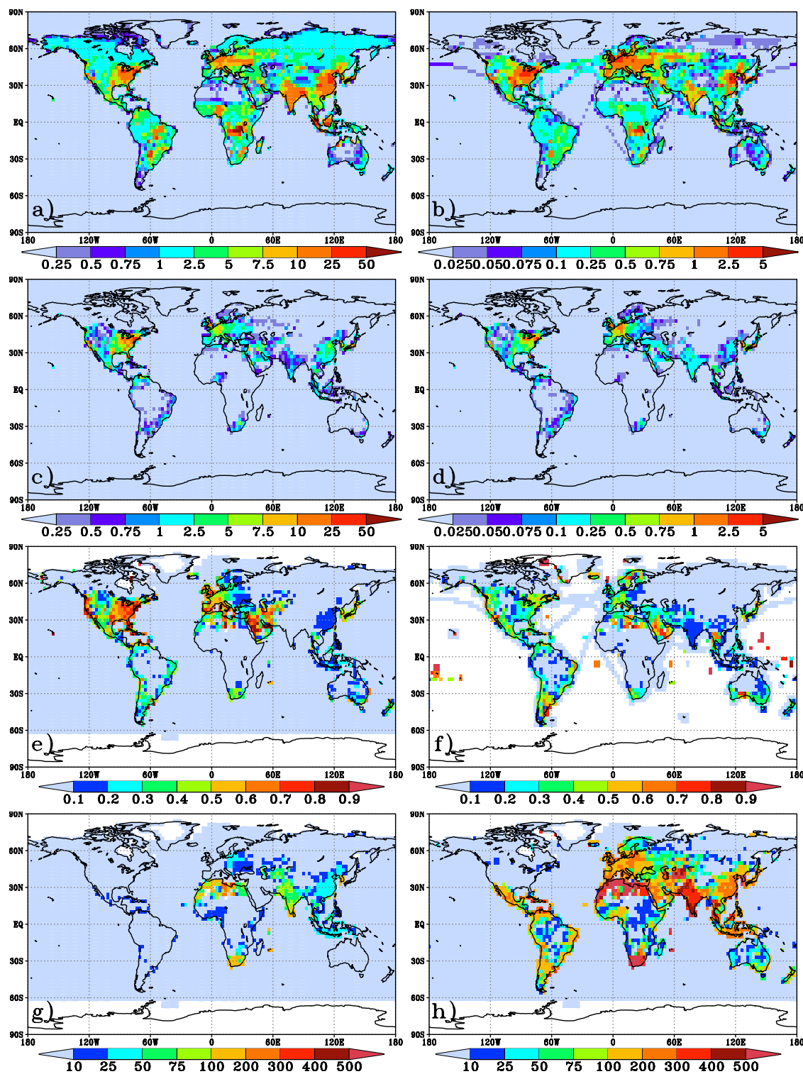
Figure 1. Distributions (in 10^{10} molecules \text{cm}^{-2} \text{s}^{-1} ) of (a) CO and (b) NO x total emissions, (c) CO and (d) NO x emissions due to road traffic only, (e) CO road/total emission ratio, (f) NO x road/total emission ratio, (g) CO emissions difference (%) between cases 5 and 2 and (h) CO emissions difference (%) between cases 6 and 2. See text for further details.
