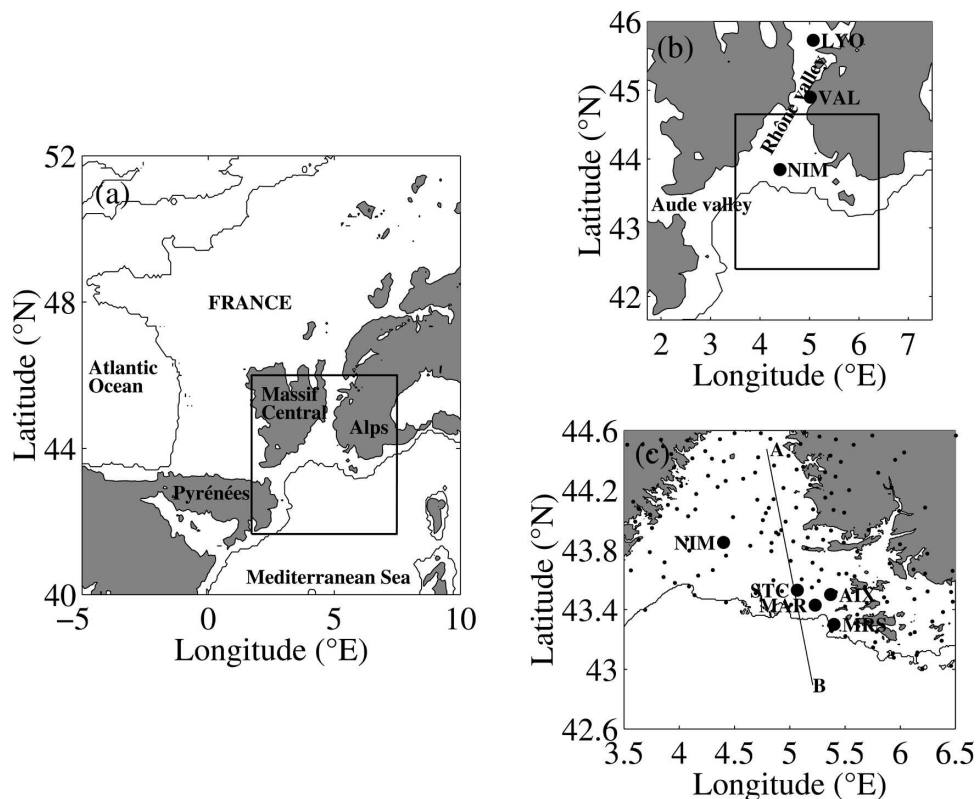
FIG. 1. (a) Map of France with the topography shaded in gray when higher than 500 m above sea level. The rectangle displays the large domain (hereafter called domain 1) of the Méso-NH simulations. (b) Domain 1 of the simulation with its nested smaller domain (hereafter called domain 2) in the rectangle. The acronyms NIM, LYO, and VAL stand for the city names Nîmes, Lyon, and Valence, respectively. (c) Domain 2 of the Méso-NH simulation. The solid line corresponds to a segment of the flight track of the DLR Falcon 20 carrying the Doppler lidar WIND on 22 Jun 2001, along which a cross section of the wind field is shown in Fig. 7 (A and B indicate the limits of the segment). The flight altitude is 6.5 km and the aircraft speed is about 170 \text{ m s}^{-1} . The dots indicate the locations of the operational meteorological surface stations operated by Météo-France. The acronyms AIX, MAR, MRS, NIM, and STC correspond to the city names Aix-en-Provence, Marignane, Marseille, Nîmes, and Saint Chamas, respectively.
