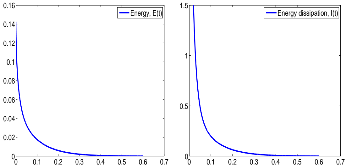
FIG. 6. Thermal equilibrium at the boundary in 2-D: evolution of the numerical energy and its numerical dissipation in the linear case
