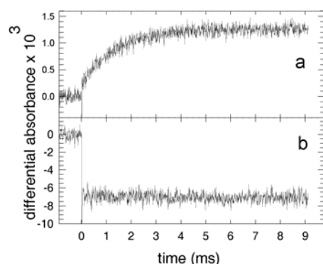
Figure 3 Transient signals obtained for (dT)_{20} at 325 nm (a) and 290 nm (b). Excitation density at 266 nm: 1.2 \text{ MW/cm}^2 . None of the signals is affected when oxygen is bubbled in the solution.
