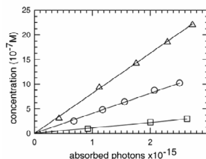
Figure 4. Concentrations of the photo-induced species as a function of the number of absorbed photons per pulse: TMP triplet at zero time (circles), T<>T in (dT)_{20} (triangles) and (6-4) in (dT)_{20} (squares). The TMP triplet and (6-4) concentrations are determined for \epsilon_{\text{max}} values of 2300 \text{ M}^{-1}\text{cm}^{-1} , 10 and 4600 \text{ M}^{-1}\text{cm}^{-1} , 14 respectively. The T<>T concentrations are calculated considering that the formation of one dimer results to the depletion of two thymine residues and that the \epsilon of (dT)_{20} at 290 nm is 1780 \text{ M}^{-1}\text{cm}^{-1} per base 15
