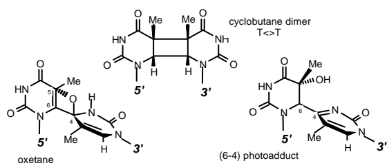
Figure 1 Structure of the dimeric thymine photoproducts.
