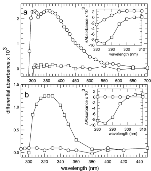
Figure 2. Transient absorption spectra recorded at 200 ns (a) and 10 ms for TMP (circles) and at (dT) 20 (squares). Excitation density at 266 nm: 1.2 MW/cm 2 .
