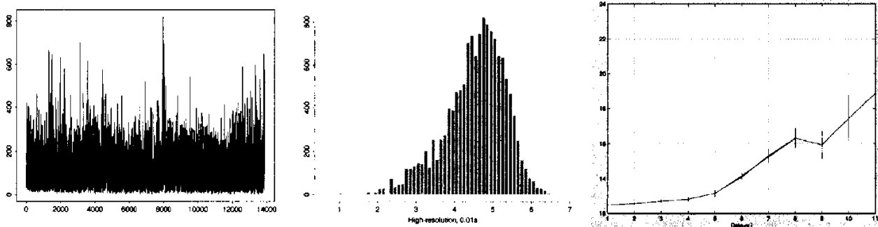
Figure 4.15. Munich hi .01s: left ) trace, middle ) histogram of log traffic rate, and right ) wavelet regression estimation of the Hurst exponent H = .101 \pm .04 .
