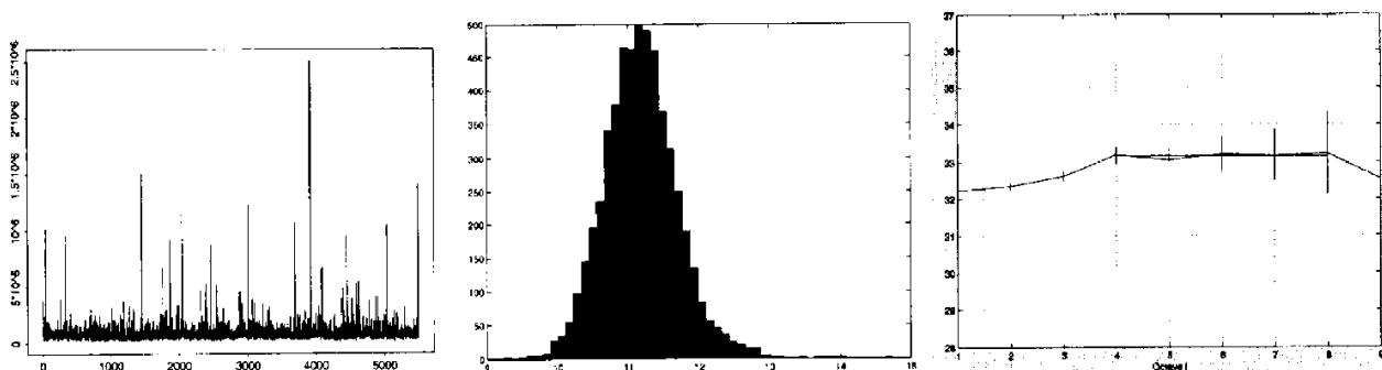
Figure 4.8. UCB, traffic rate 2 second blocks, ( \hat{\gamma}_T = .05 \pm .17 left) trace, middle) histogram of log traffic rate, and right) wavelet regression estimation of the Hurst exponent, \hat{H} = 0.50 \pm .01 .
