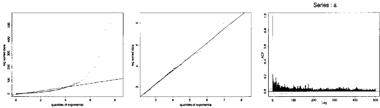
Figure 4.2. BUburst. Inter-arrival times of bursts: left ) qq-plot against exponential distribution, middle ) Pareto fit for the 400 largest values (last 10 %), ( \alpha = 1.54 ), right ) autocorrelation function.
