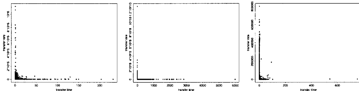
Figure 4.19. Plot of transfer times against transfer rates for left ) the BUburst trace, middle ) the UCB trace, and right ) and the Ericsson trace.
