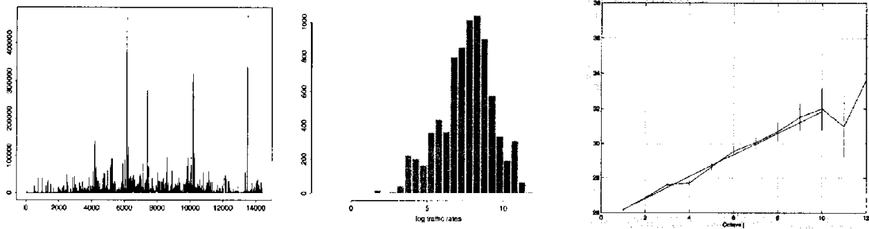
Figure 4.4. BUburst 1s. Traffic rates: left ) trace, middle ) histogram of log traffic rates; right ) wavelet regression estimation of the Hurst parameter, H = 0.81 \pm .01 .
