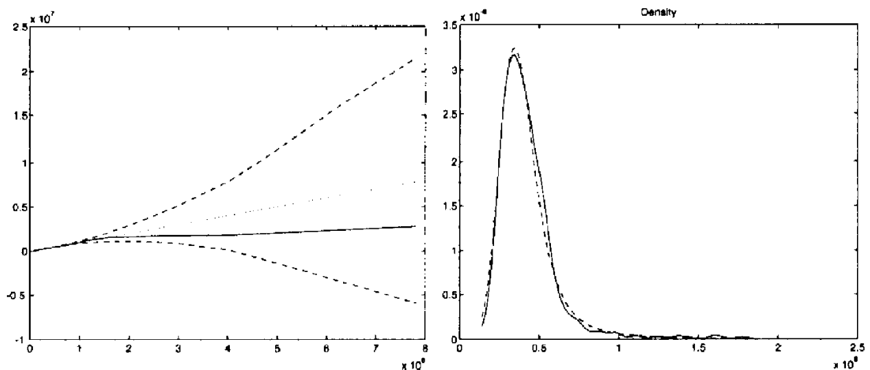
Figure 4.10. UCB 10s traffic rate: left ) qqplot (solid line) against estimated stable distribution (dashed lines are the confidence interval), and right ) density estimate and density of estimated stable distribution \alpha = 1.52 \pm .02 , \beta = 1.00 \pm .00 , \sigma = 86000 \pm 1200 , \delta = 438000 \pm 2300 .
