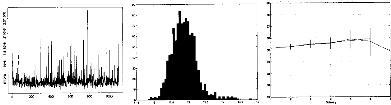
Figure 4.9. UCB, traffic rate 10 seconds blocks, ( \hat{\gamma}_T = .05 \pm .17 ) left ) trace, middle ) histogram of log traffic rate, and right ) wavelet regression estimation of the Hurst exponent, \hat{H} = 0.58 \pm .03 .
