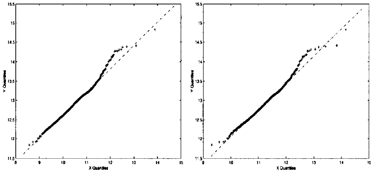
Figure 4.11. UCB: comparison of the distribution of traffic rate over time blocks of varying lengths: left ) qqplot of log traffic rate for 1 second blocks against 10 second blocks and right ) qqplot of log traffic rate for 2 second blocks against 10 second blocks.
