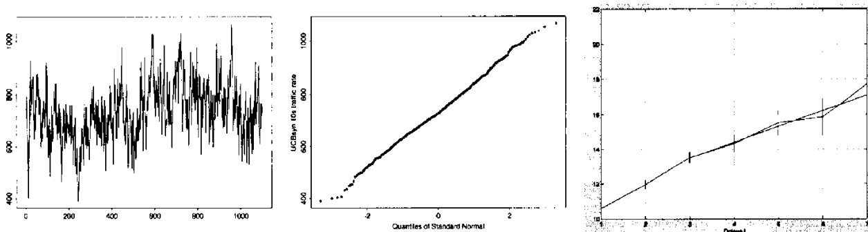
Figure 4.17. UCB syn 10s traffic rates: left ) trace, middle ) qqplot vs. normal variable, right ) wavelet regression estimation of the Hurst parameter H = .95 \pm .07 .
