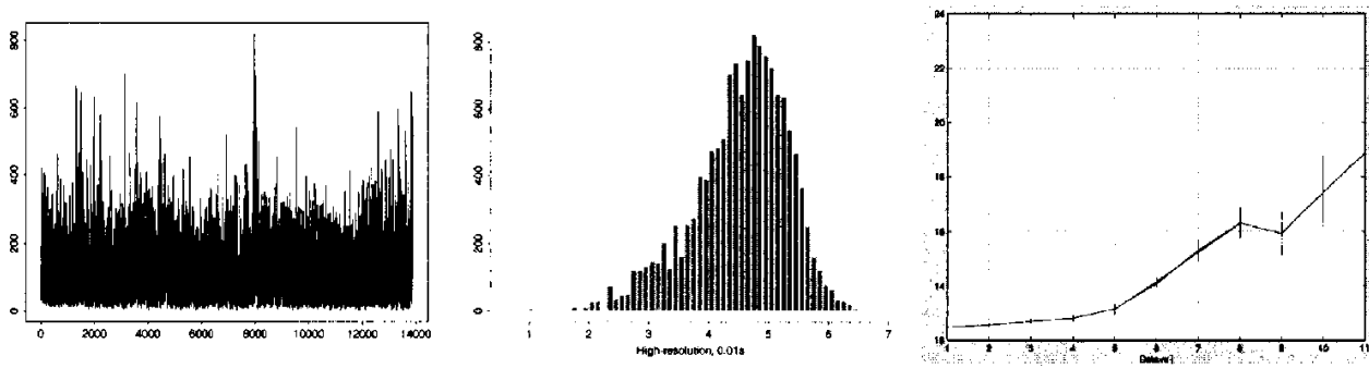
Figure 4.15. Munich hi .01s: left ) trace, middle ) histogram of log traffic rate, and right ) wavelet regression estimation of the Hurst exponent H = .101 \pm .04 .
