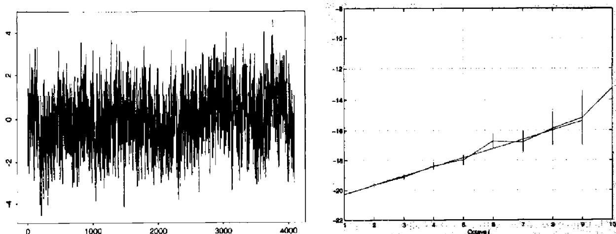
Figure 3.2. Synthetic trace from fGn, H = .8 , used as the traffic rate: left ) the traffic rate, and right ) wavelet regression estimation of Hurst parameter, \hat{H} = .81 \pm .01 .
