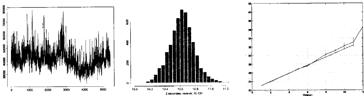
Figure 4.12. Munich lo, RX: left ) trace, middle ) histogram of log traffic rate, and right ) wavelet regression estimation of the Hurst exponent H = .97 \pm .01 .
