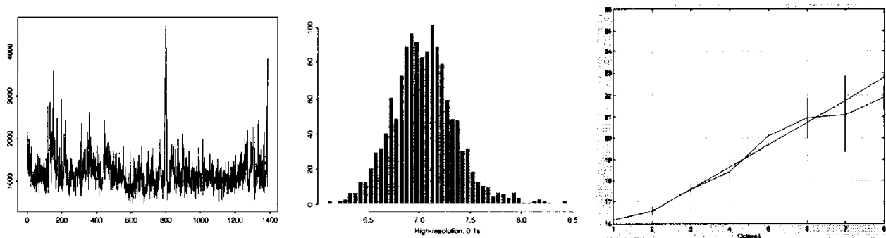
Figure 4.14. Munich hi .1s: left ) trace, middle ) histogram of log traffic rate, and right ) wavelet regression estimation of the Hurst exponent H = 1.02 \pm .03 .
