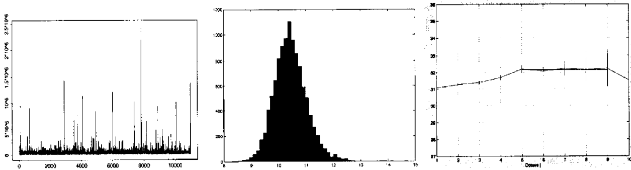
Figure 4.7. UCB, traffic rate 1 second blocks, ( \hat{\gamma}_T = 43 \pm .06 left) trace, middle) histogram of log traffic rate, and right) wavelet regression estimation of the Hurst exponent, \hat{H} = 0.50 \pm .04 .
