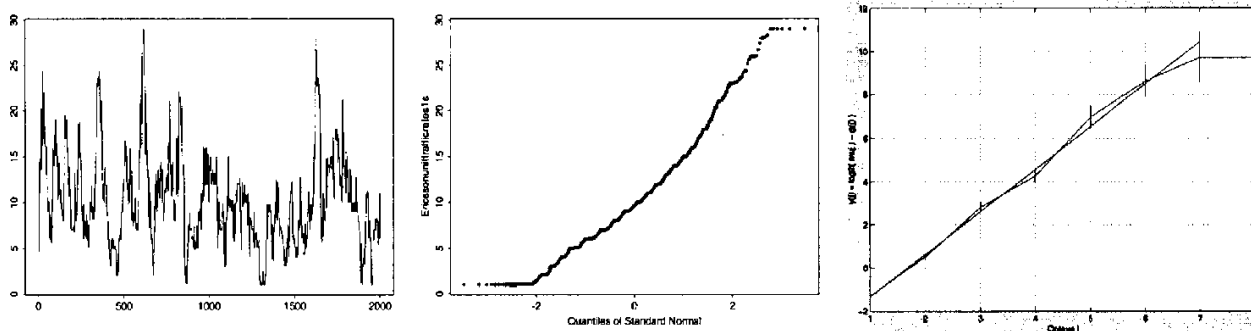
Figure 4.18. Eri syn 1 s traffic rates left ) trace, middle ) qqplot vs. normal variable, right ) regression estimation of the Hurst parameter H = 1.48 \pm .02 .
