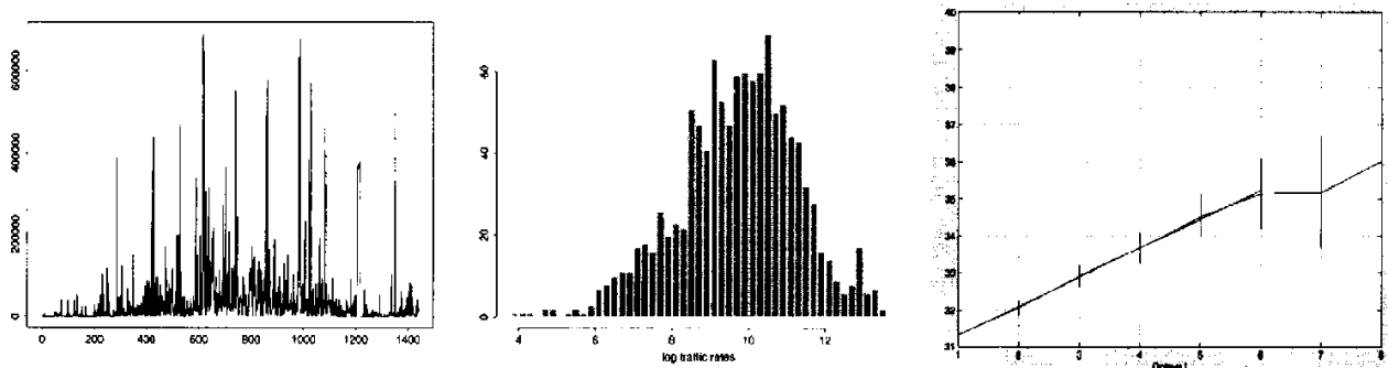
Figure 4.3. BUburst 10s. Traffic rates: left ) trace, middle ) histogram of log traffic rates; right ) wavelet regression estimation of the Hurst parameter H = .89 \pm .02 .
