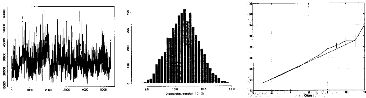
Figure 4.13. Munich lo, TX: left ) trace, middle ) histogram of log traffic rate, and right ) wavelet regression estimation of the Hurst exponent H = .89 \pm .01 .
