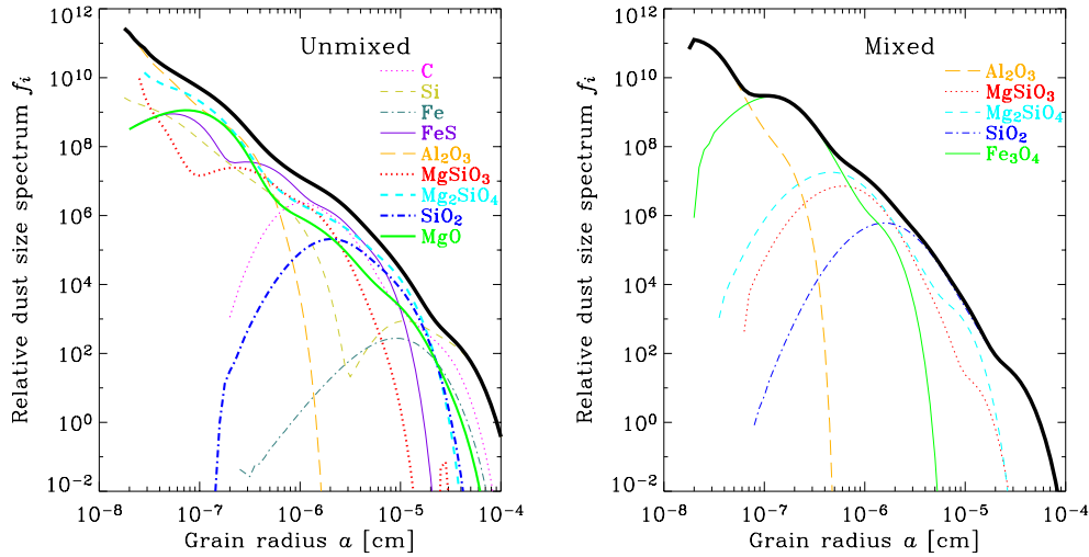
Figure 1. Dust size distributions of the SN II model with the progenitor mass of 20M_{\odot} by Nozawa et al. (2003). The thick lines are the total dust size distribution function. The labels ‘unmixed’ and ‘mixed’ indicate the adopted assumption of the mixing of elements in the ejecta. We assumed 20M_{\odot} as a representative for the SN progenitor mass in this work.
