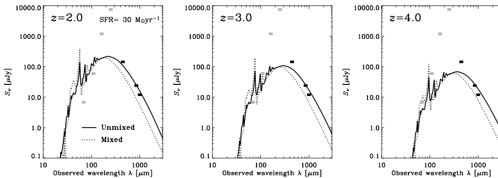
Figure 12. The expected flux densities of an LBG. In this figure we set the galaxy burst age of t = 10^8 \text{ yr} . Confusion limits of Herschel and detection limits of ALMA 8-h survey are also shown by grey and black thick horizontal lines, respectively.
