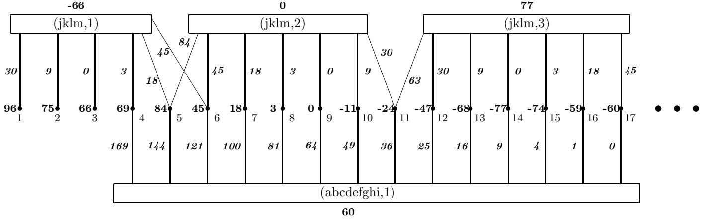
FIG. 6 – Bipartite graph for d_a = d_b = \dots d_i = 1, d_j = d_k = \dots d_m = 6 and weights for the min-sum-sqr problem
