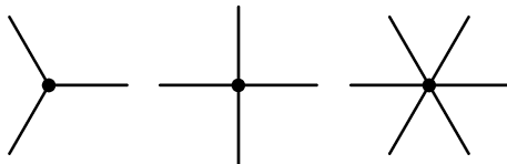
FIG. 8: Vertices with 3 and 4 legs obtained from \mathcal{S}_1 , i.e. , with 1 replica.
