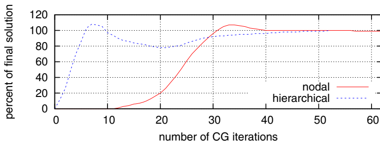
Fig. 5. Convergence speed in a static solver
