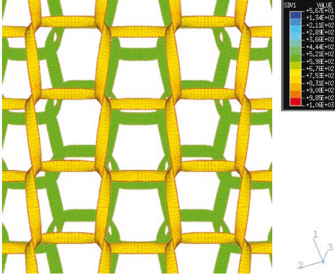
Figure 6. Bi-axial test. Initial and Deformed state
