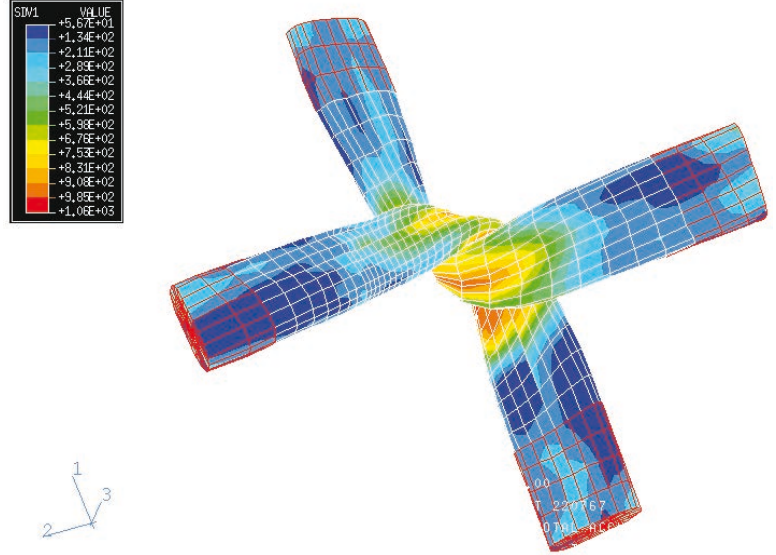
Figure 7. Transverse Young's moduli (MPa) at the end of the motion
