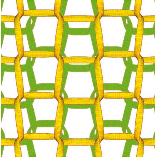
Figure 6. Bi-axial test. Initial and Deformed state
