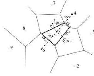
Fig. 3. Parameters involved in Laplace interpolant computations
