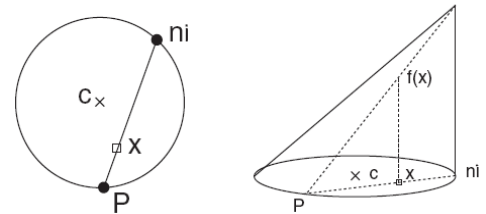
Fig. 5. Conical function.
