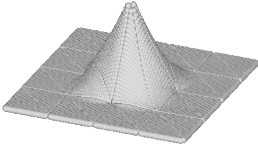
Fig. 2. Sibson interpolant
