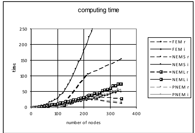
Fig. 8. Computing time comparison
