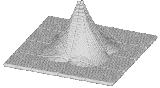
Fig. 4. Laplace interpolant
