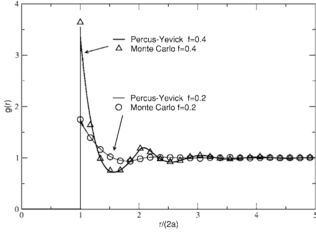
Fig. 2. Pair distribution function for two different densities. There is excellent agreement between Monte Carlo simulations (circles and triangles) and Percus–Yevick hard-sphere distribution functions (solid curves).
