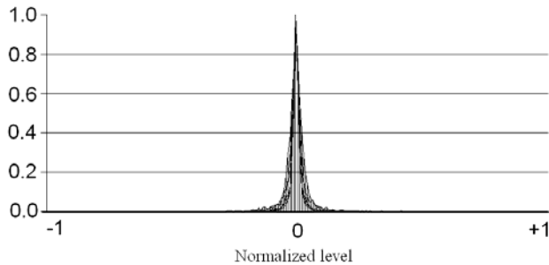
Fig. 4. The probability density function (PDF) of the highband Wavelet coefficients (horizontal, vertical and both direction).
