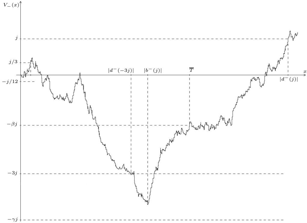
Figure 2: Example of \omega \in \Theta^-(j)
