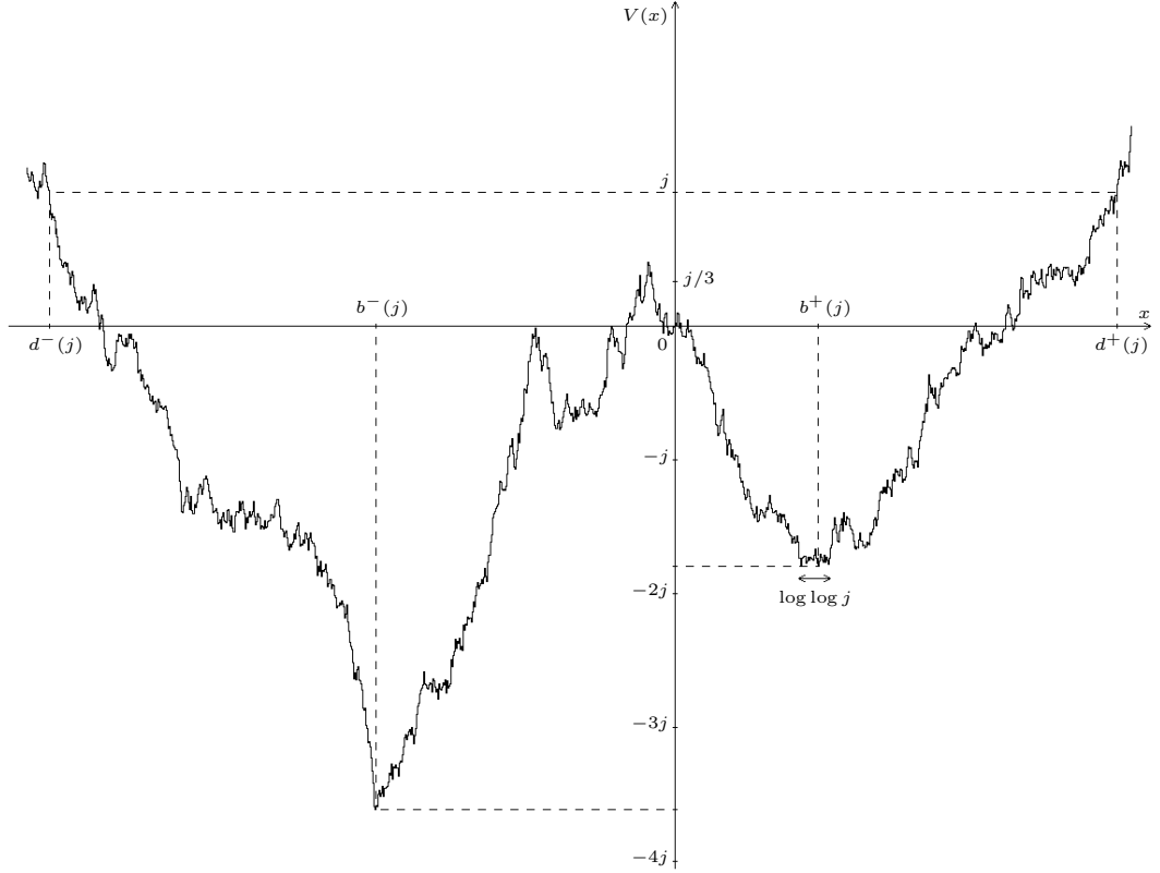
Figure 1: Example of \omega \in E^+(j) \cap E^-(j)
