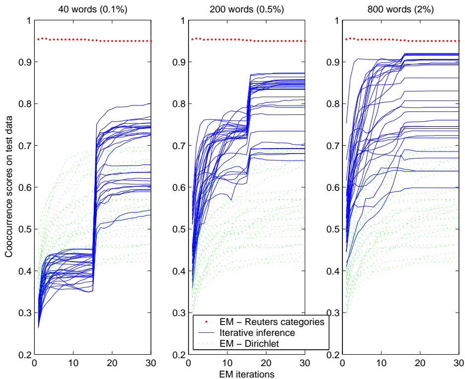
Figure 7: Evolution of cooccurrence scores on test data with different vocabulary sizes. The first 15 iterations are conducted on reduced vocabularies (the size of which is reported on top the figures), while the last 15 are use the complete vocabulary.
