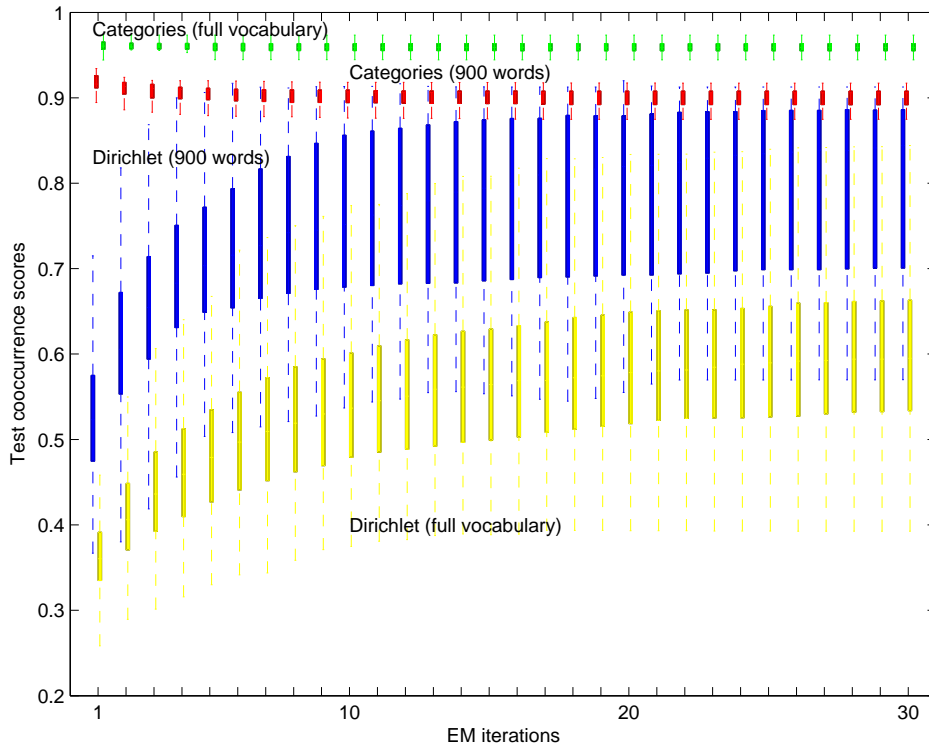
Figure 5: Evolution of test cooccurrence scores over the EM iterations with a vocabulary of size 900.
