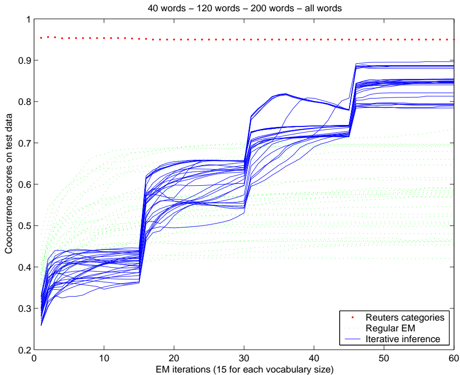
Figure 8: Evolution of cooccurrence scores over the different steps of an iterative algorithm (30 runs on the same fold).
