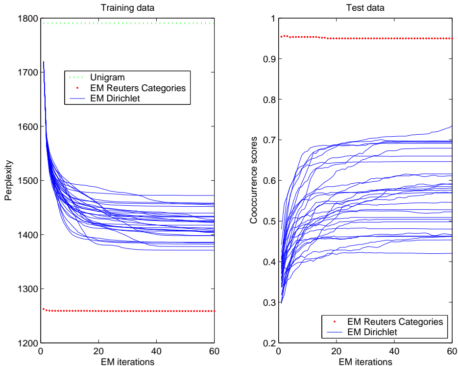
Figure 3: Evolution of Perplexity and Cooccurrence scores over the EM iterations for different Dirichlet initializations for the first fold.
