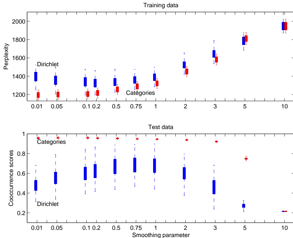
Figure 4: Evolution of training perplexity and test cooccurrence scores over the smoothing parameter \lambda_\beta - 1 .
