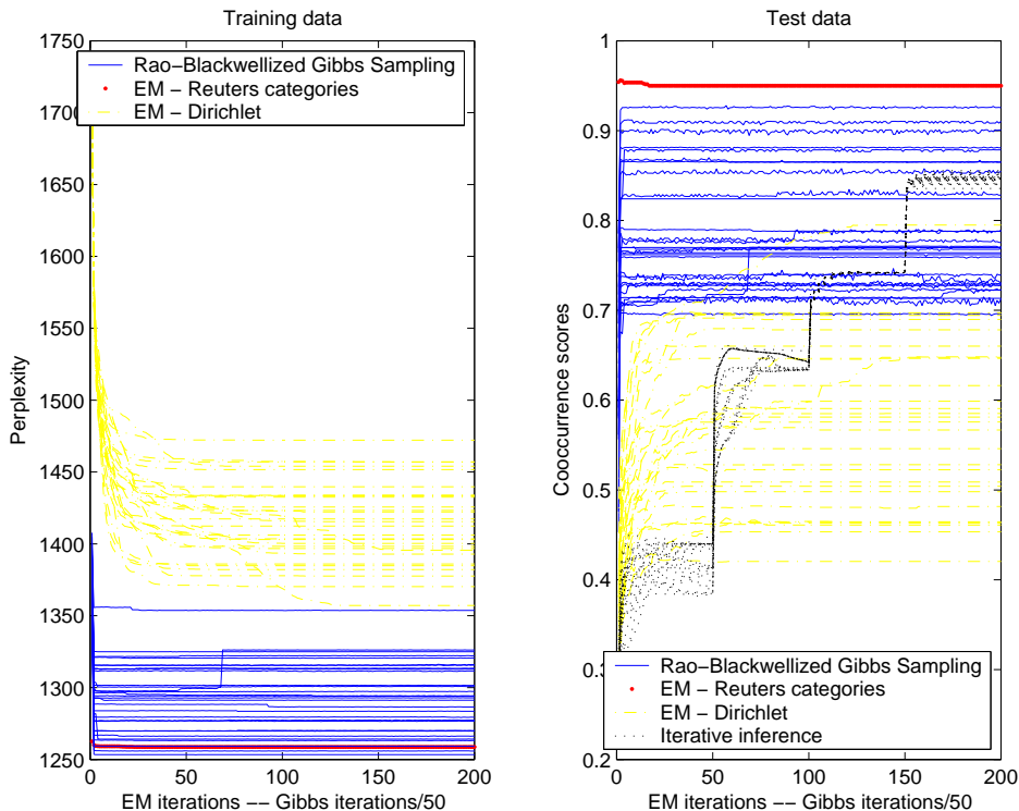
Figure 11: Evolution of the different measures for Rao-Blackwellized Gibbs Sampling
