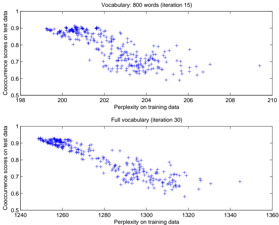
Figure 9: Correlation between training perplexity and test cooccurrence scores.
