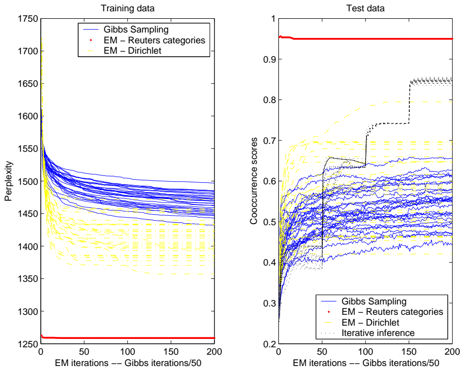
Figure 10: Evolution of perplexity and cooccurrence scores over the EM-Gibbs Sampling iterations.
