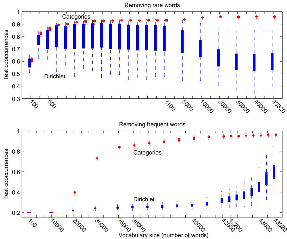
Figure 6: Evolution of test cooccurrence scores over the size of vocabulary with two different strategies: discarding most rare words or discarding most frequent words.
