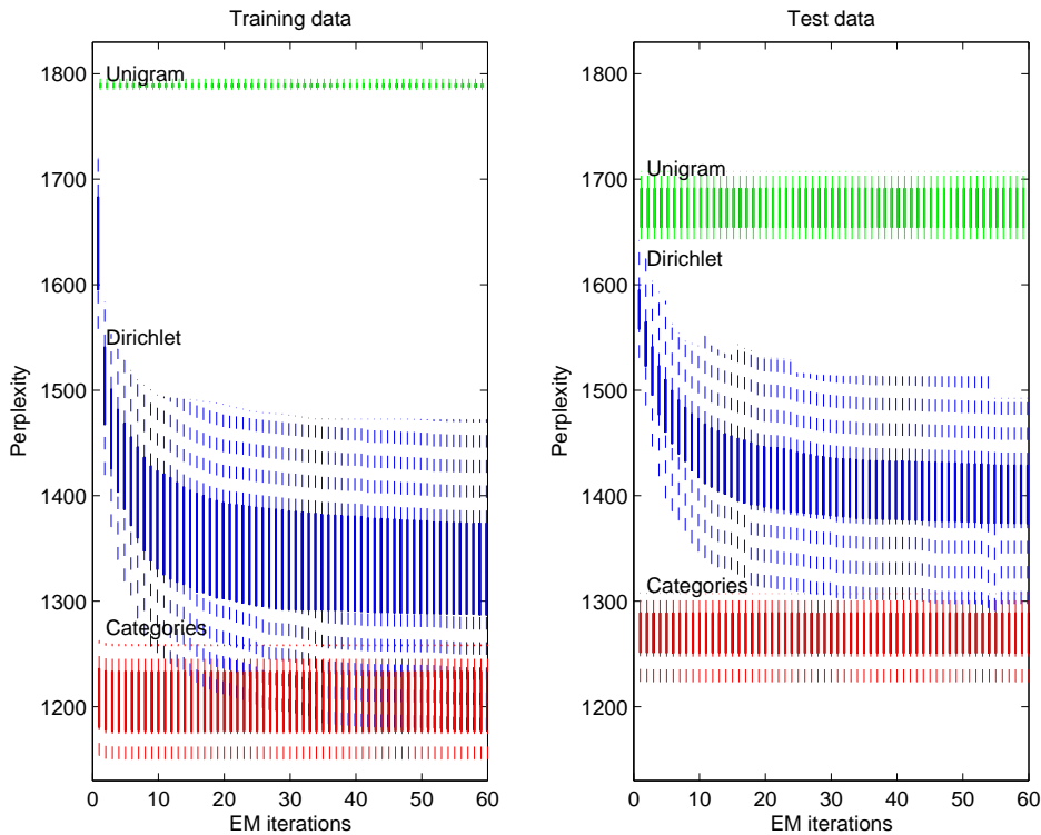
Figure 2: Evolution of Perplexity on training and test data over the EM iterations.
