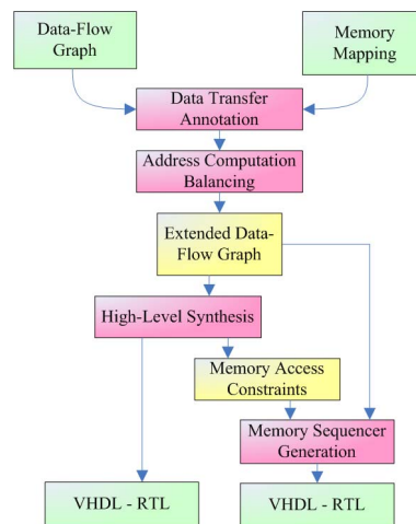
Figure 1. Design Flow
