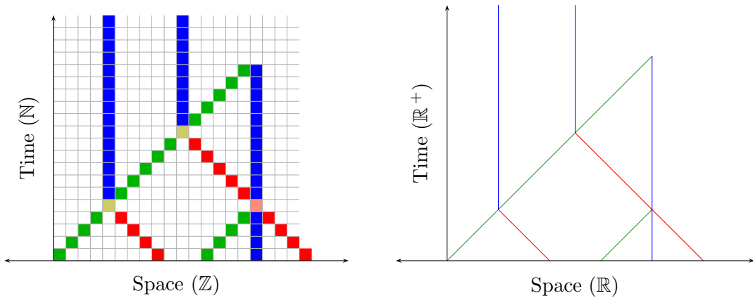
Figure 1: Space-time diagram of a cellular automaton and its signal machine counterpart.
