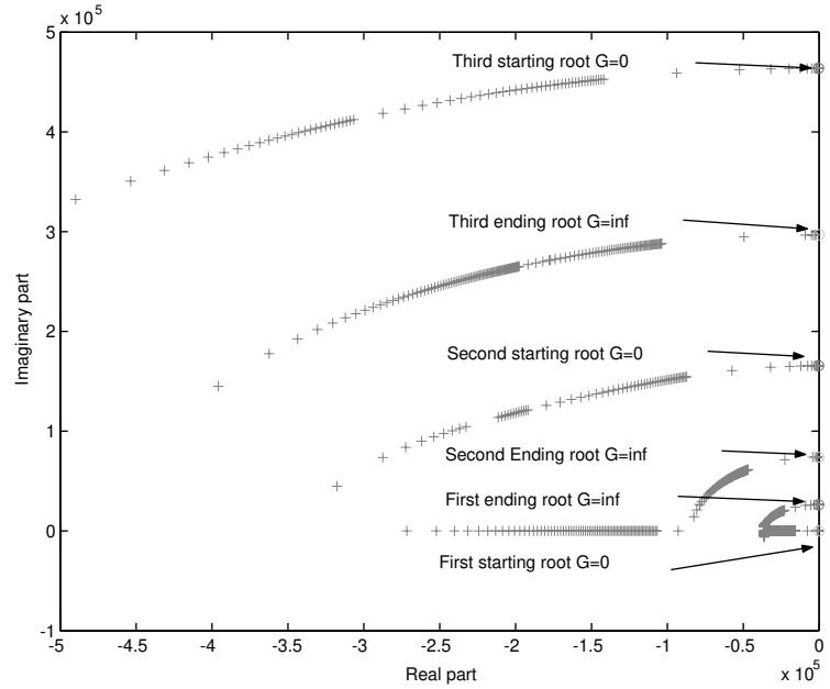
Fig. 11. First three theoretical roots locus in the complex plane.
