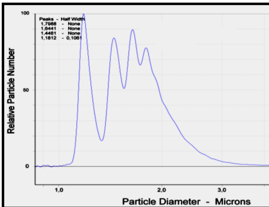
Figure 3 : Disc centrifuge characterization ( \%(\text{PVP})=30\% , \phi_{\text{int}}=17\% , shear rate 3124 \text{ s}^{-1} ).
