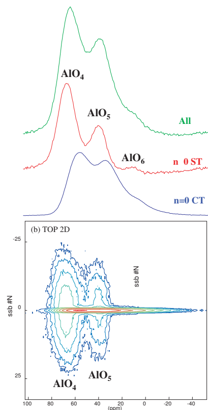
Fig. 5. (a) ^{27}\text{Al} 1D one pulse MAS, (b) TOP spectrum, and (c) Projections of a 50% \text{SiO}_2 - 40% \text{Al}_2\text{O}_3 - 10% \text{CaO} glass [29] acquired at 17.6 T while spinning at 31258 Hz (1 MHz spectral width, 1\mu\text{s} pulse \pi/6 1s recycle time 40 scans). The N=0 cross-section shows the Central Transition spectrum and the N \neq 0 sum is the satellite transition spectrum showing enhanced resolution with the \langle 3/2 \rangle transitions mostly broadened by the distribution of isotropic chemical shift.
