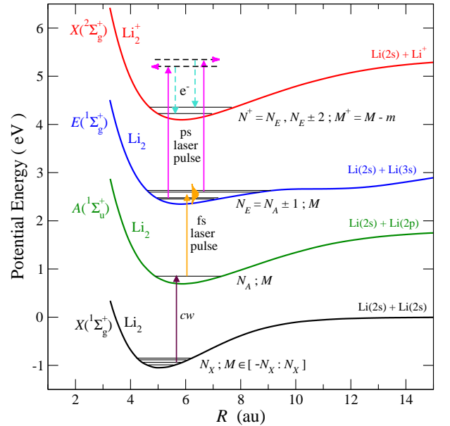
FIG. 1: (Color online) Three step “preparation-pump-probe” scheme proposed to store classical information in the phases of a rotational wavepacket in the E(1\Sigma_g^+) electronic state of the \text{Li}_2 molecule, and to read it in the photoelectron spectrum recorded in the last step which consists in a picosecond photoionization experiment. The potential energy curves of the X , A and E electronic states of \text{Li}_2 are shown as a function of the internuclear distance R as black, green and blue solid lines respectively. The potential curve associated with the ground electronic state of \text{Li}_2^+ is shown as a red solid line. Their associated molecular rotational quantum numbers are denoted by N_X , N_A , N_E and N^+ , while M and M^+ denote their projection on the electric field polarization axis.
