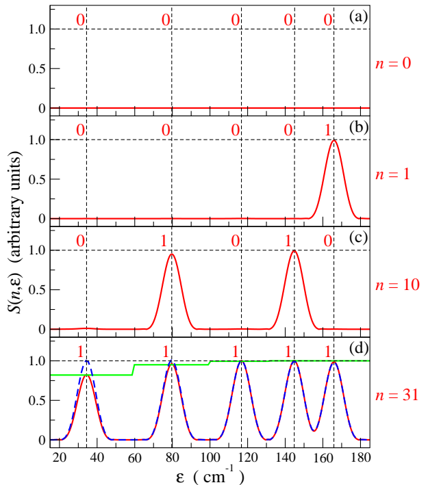
FIG. 5: (Color online) Photoelectron spectra calculated using five initial vibrational states ( v_E = 0 \dots 4 ) with a coherent superposition of two rotational levels ( N_E = 1 and N_E = 3 ) as a function of energy \varepsilon . The pulse duration is \tau = 2.5 ps and the laser wavelength is 699.6 nm. The solid red lines show the signal difference S(n, \varepsilon) = P(n, \varepsilon) - P(0, \varepsilon) when the integer values n = 0 (panel a), 1 (panel b), 10 (panel c) and 31 (panel d) are stored in the phase difference between the N_E = N_A \pm 1 rotational components of the initial wavepacket. The step function shown as a green solid line in panel (d) represents the vibrational Franck-Condon factors \mathcal{F}(\varepsilon) = \langle v_+ | v_E \rangle associated with the different photoelectron peaks. The ratio S(n, \varepsilon)/\mathcal{F}(\varepsilon) is shown in panel (d) as a blue dashed-line.
