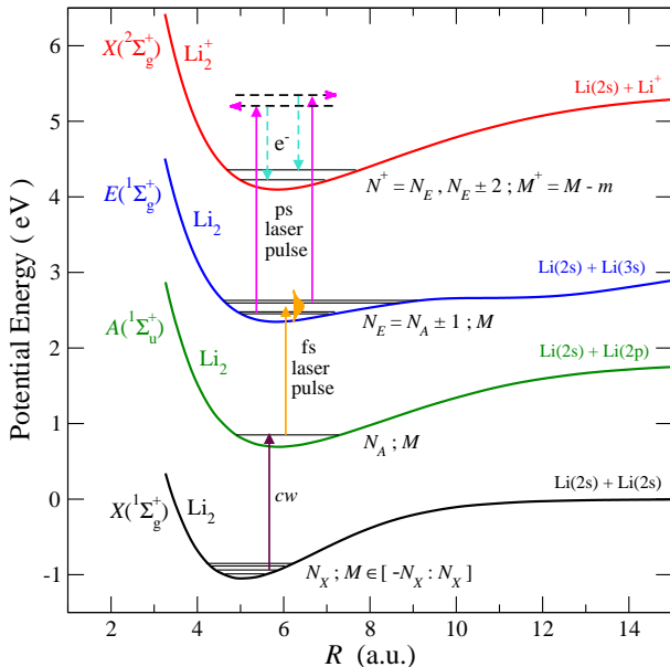
FIG. 1: (Color online) Three step “preparation-pump-probe” scheme proposed to store classical information in the phases of a rotational wave packet in the E ( 1\Sigma_g^+ ) electronic state of the \text{Li}_2 molecule, and to read it in the photoelectron spectrum recorded in the last step which consists of a picosecond photoionization experiment. The potential energy curves of the X , A and E electronic states of \text{Li}_2 are shown as a function of the internuclear distance R as black, green and blue solid lines respectively. The potential curve associated with the ground electronic state of \text{Li}_2^+ is shown as a red solid line. Their associated molecular rotational quantum numbers are denoted by N_X , N_A , N_E and N^+ , while M and M^+ denote their projection on the electric field polarization axis.
