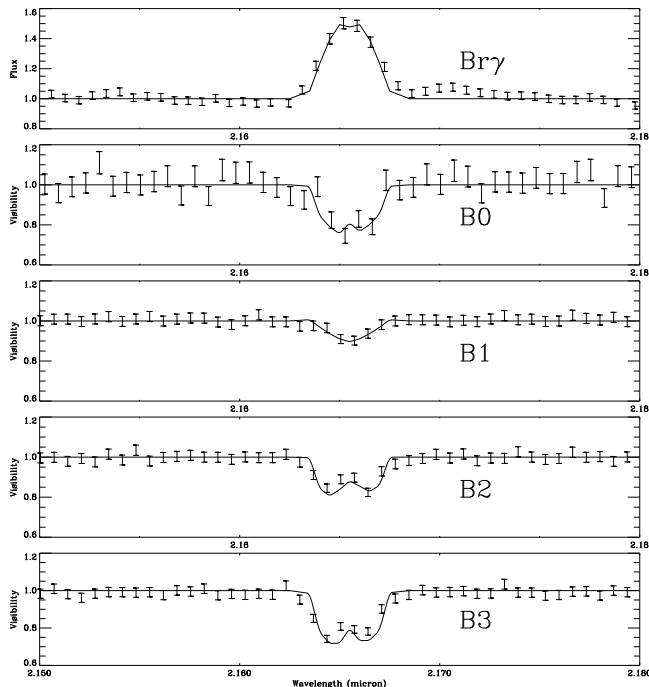
Fig. 10. Differential visibility across the Bry line profile for the B_0 , B_1 , B_2 and B_3 baselines. The first picture from the top is the Bry line profile. The plain line are the fits we obtain with SIMECA from our best model whereas the VLTI/AMBER data are the points with error bars.
