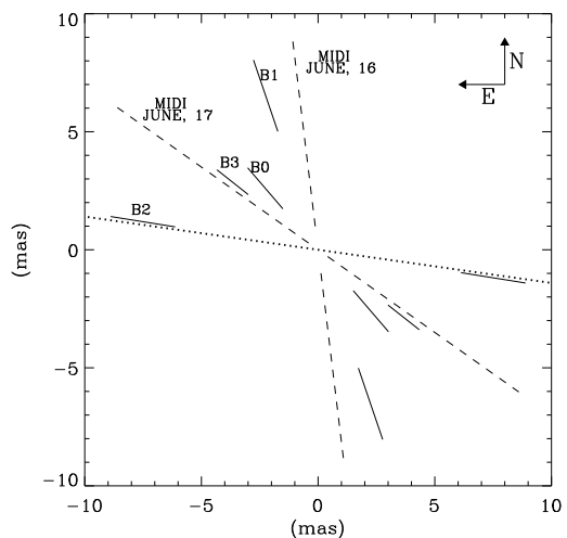
Fig. 2. \alpha Arae (unresolved star + uniform disc) model diameters (in mas) dependence on the baseline position angle. Full line: AMBER measurements in the continuum at 2.1\mu\text{m} . Dashed lines: MIDI measurements. The length of the plot corresponds to the values of the error bars (note the very large error bars for the MIDI data). The dotted line is the direction of the major-axis of the envelope estimated from polarization measurements (PA= 172^\circ ) obtained by McLean & Clarke 7 (9) and Yudin et al. 9 (9)
