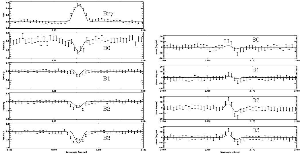
Fig. 15. \alpha Arae differential visibilities (left) and phases (right) across the \text{Br}\gamma line profiles for the B_0 , B_1 , B_2 and B_3 baselines. The plain line are the fits we obtain with SIMECA from a rotating and expanding scenario described in section 6.6 whereas the VLT/AMBER data are the points with error bars
