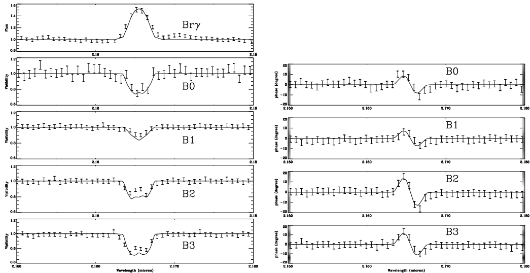
Fig. 16. \alpha Arae differential visibilities (left) and phases (right) across the \text{Br}\gamma line profiles for the B_0 , B_1 , B_2 and B_3 baselines. The plain line are the fits we obtain with SIMECA from the model 3 described in section 4.3.2 and section 6.6 whereas the VLT/AMBER data are the points with error bars
