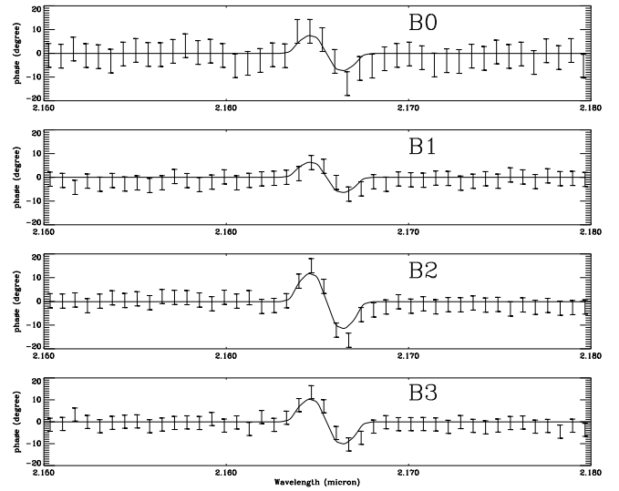
Fig. 11. Phase of the visibility across the Bry line profile for the B_0 , B_1 , B_2 and B_3 baselines. The plain line are the fits we obtain with SIMECA from our best model whereas the VLTI/AMBER data are the points with error bars.
