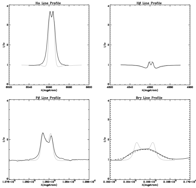
Fig. 9. Line profiles modeled with the SIMECA code using a thin disk + polar wind scenario. Modeled profiles are dotted lines whereas observed ones are in plain line. For Bry we have convoluted the modeled profile (dotted line) obtain with SIMECA with a 15 \text{ \AA} gaussian, corresponding to the AMBER spectral resolution of 1500 . The convoluted Bry profile we obtain is the dashed line superimposed with the observed one (plain line).
