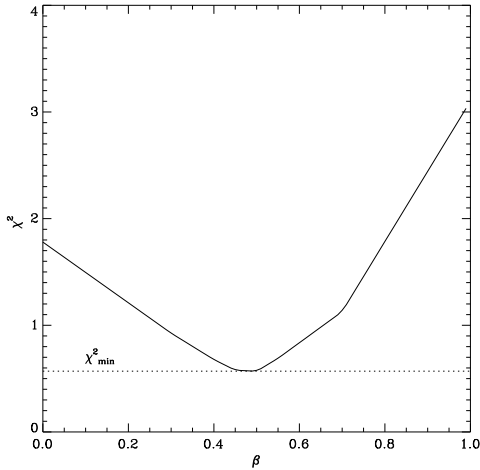
Fig. 14. \chi^2 from our models and the AMBER data plotted as a function of the \beta parameter. \chi^2_{min} is the minimum value obtained for a model with \beta=0.48 which is very close to the Keplerian rotation ( \beta=0.5 ).
