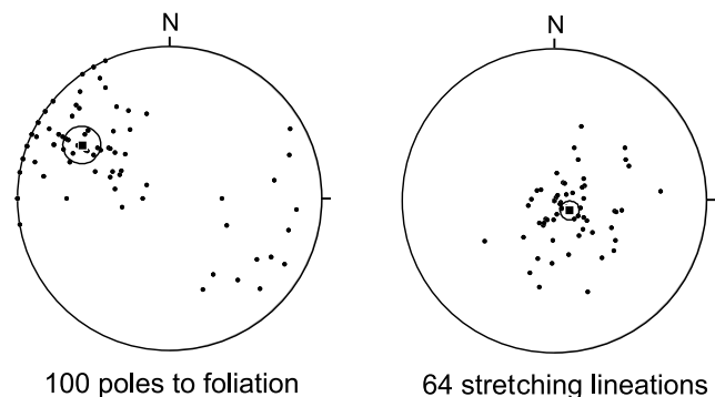
Figure 4. Stereograms (equal angle, lower hemisphere) showing distribution of foliation poles and stretching lineations in the studied part of the TNB. Mean foliation pole (square) plunges 22.4° in the N301.4° direction (95% confidence cone angle is 9.8°). Mean lineation (square) plunges 76.5° in the N122.4° direction (95% confidence cone angle is 7.1°).
