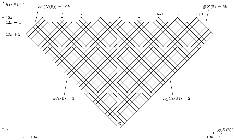
FIGURE 1. Diagram of possible values for (\chi(X(\mathbb{R})), h_*(X(\mathbb{R})))
