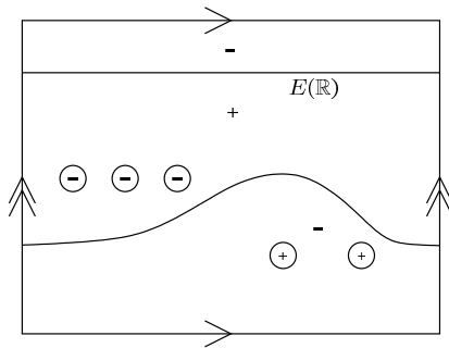
FIGURE 2. Real scheme \langle 2 \mid 3 \rangle
