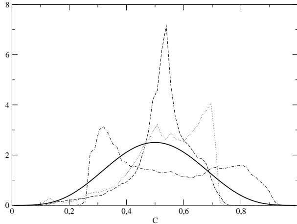
Figure 6: Comparisons between a \beta law (solid line) and several arbitrary chosen FDFs, for \bar{c} = 0.5 \pm 0.01 and \alpha = 0.0125 \pm 0.0005 .
