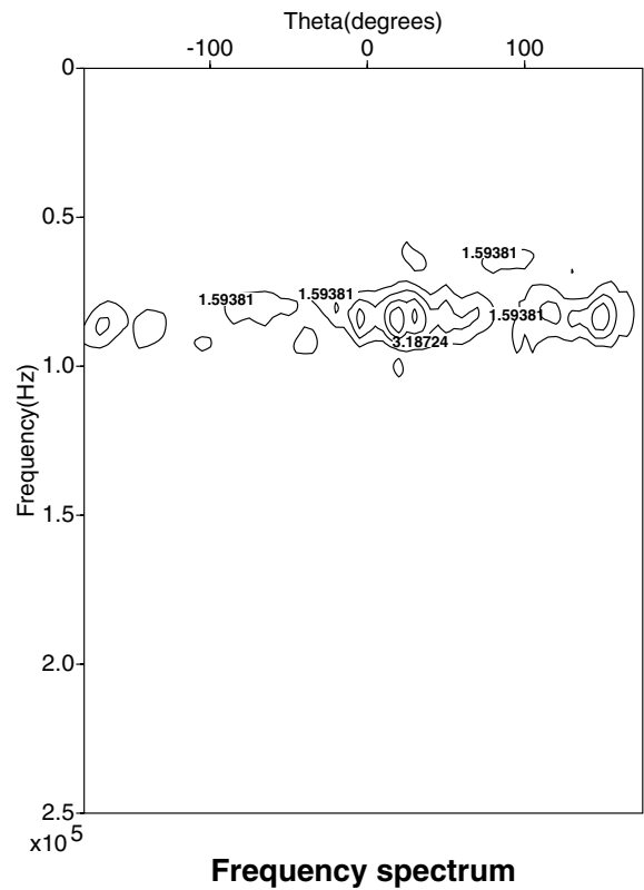
Figure 19. Frequency spectrum of the data in the azimuthal–frequency plane after wavelet filtering. The main energy is located around 0^\circ where the target is expected, with an energy ratio of 3. This result allows us to demonstrate that the other detected signals are some residuals as a result of weak multiple reflections of the target and the ambient noise.
