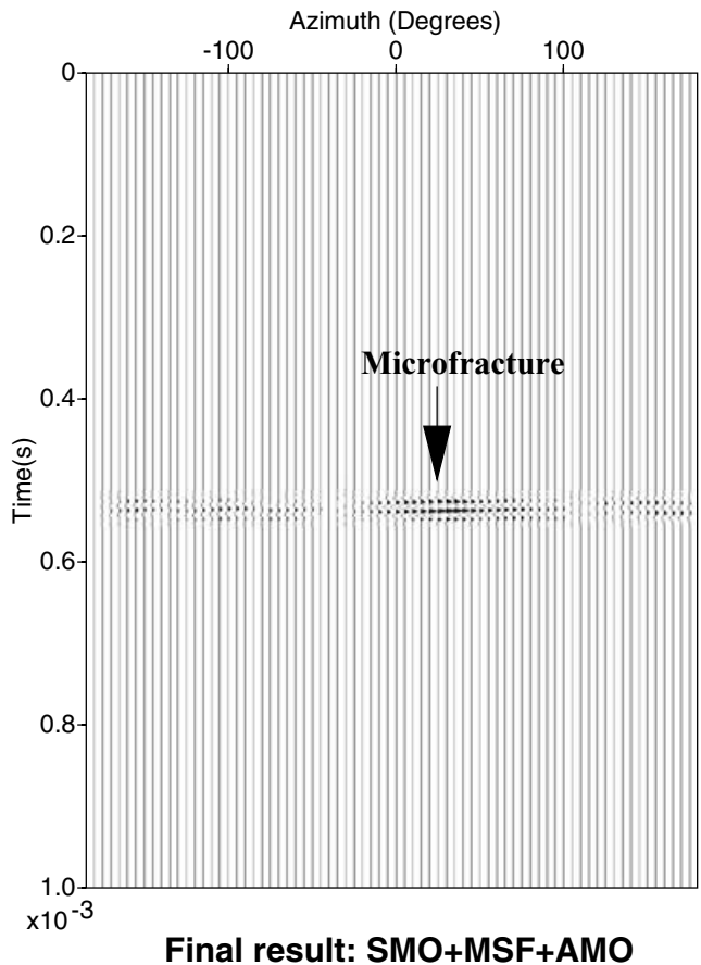
Final result: SMO+MSF+AMO Figure 20. Final result obtained after Stoneley move out (SMO) and azimuthal move out (AMO) correction combined with the multiscale filtering (MSF). All borehole waves have been removed and it becomes easy to detect the position of the fracture in the azimuth–time domain.
