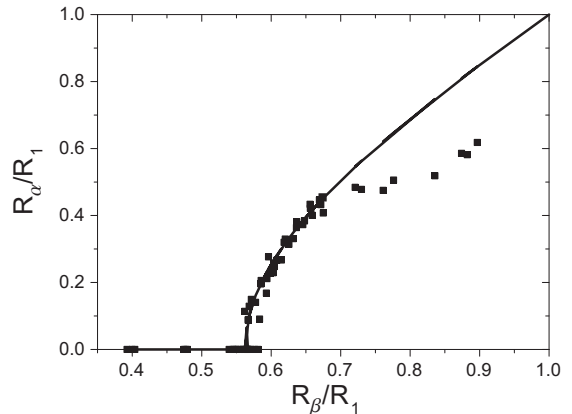
FIG. 2: Comparison between experimental data of ref. [14] (squares) and eq. (4) (full line). R_\alpha , R_\beta and R_1 are respectively the radii of the superfluid, minority and majority components. The condensate vanishes for R_\alpha = 0 at q = R_\beta^2 / R_1^2 \sim 0.32 .
