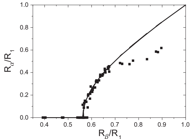
FIG. 2: Comparison between experimental data of ref. [1] (squares) and eq. (6) (full line). R_{\alpha} , R_{\beta} and R_1 are respectively the radii of the superfluid, minority and majority components. The condensate vanishes for R_{\alpha} = 0 at q = R_{\beta}^2/R_1^2 \sim 0.32 .
