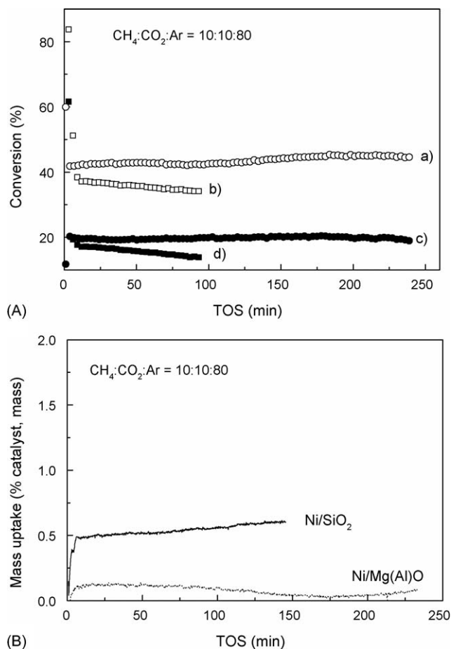
Fig. 3. (A) Changes in methane [(●) (c), (■) (d)] and carbon dioxide [(○) (a), (□) (b)] conversion vs. time on stream (min) in the TEOM reactor over Ni/SiO 2 [(□) (b), (■) (d)] and Ni/Mg(Al)O [(○) (a), (●) (c)]; (B) Mass uptake (expressed as carbon wt.% referring to the catalyst) vs. time on stream (min) for methane dry reforming in the TEOM reactor for Ni/SiO 2 and Ni/Mg(Al)O.
