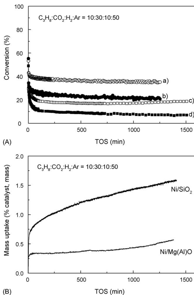
Fig. 4. (A) Changes in propane [(●) (b), (■) (d)] and carbon dioxide [(○) (a), (□) (c)] conversion vs. time on stream (min) in the TEOM reactor over Ni/SiO 2 [(□) (c), (■) (d)] and Ni/Mg(Al)O [(○) (a), (●) (b)] catalysts; (B) Mass uptake (expressed as carbon wt.% referring to the catalyst) vs. time on stream (min) for propane dry reforming in the TEOM reactor for Ni/SiO 2 and Ni/Mg(Al)O.
