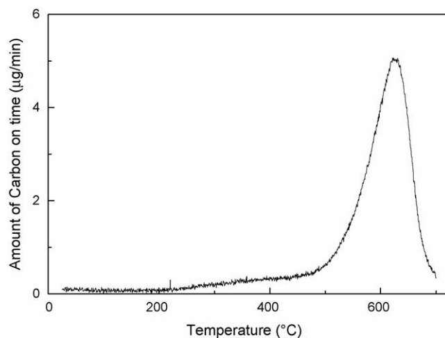
Fig. 5. Amount of carbon hydrogenated into methane during TPH experiments after TEOM methane dry reforming over Ni/Mg(Al)O for 4 h. Heating rate during the TPH experiment was 10 °C/min.
