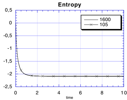
Figure 8: entropy
