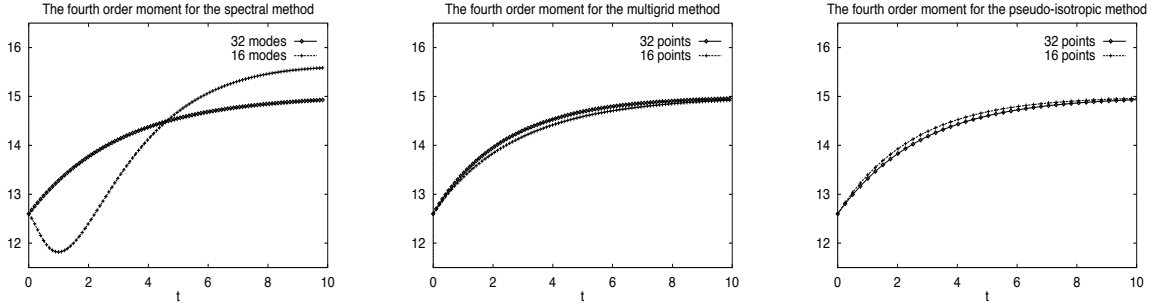
FIGURE 3. Evolution of the fourth order moment for (1) the spectral method, (2) the multigrid method, (3) the pseudo-isotropic scheme using 16^3 and 32^3 unknowns (TEST 1).
