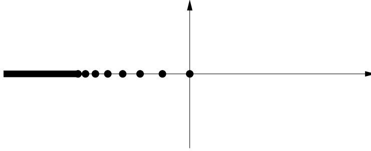
FIGURE 1. Spectrum of \mathcal{L} in L^1
