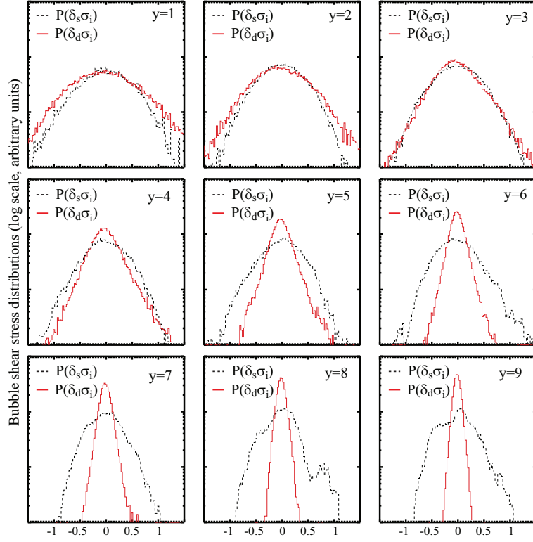
FIGURE 15. Static stress distributions P(\delta_s\sigma_i) and dynamic stress distribution P(\delta_d\sigma_i(\Delta t)) measured in the permanent regime for \Delta t = \tau_0 at different distances from the inner wall. Data are obtained from the experiment during the permanent regime.
