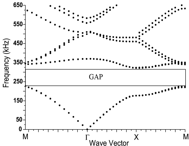
FIG. 4: Band diagram of the phononic crystal.
